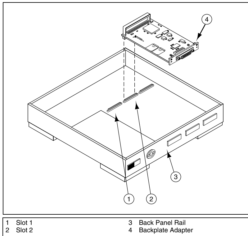
Figure 2-1. Installing the SB-GPIB/TNT or SB-GPIB
