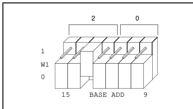
Figure 3-3. Configuration for GPIB-1014 Base Address 2000 (hex) (Default Setting)
