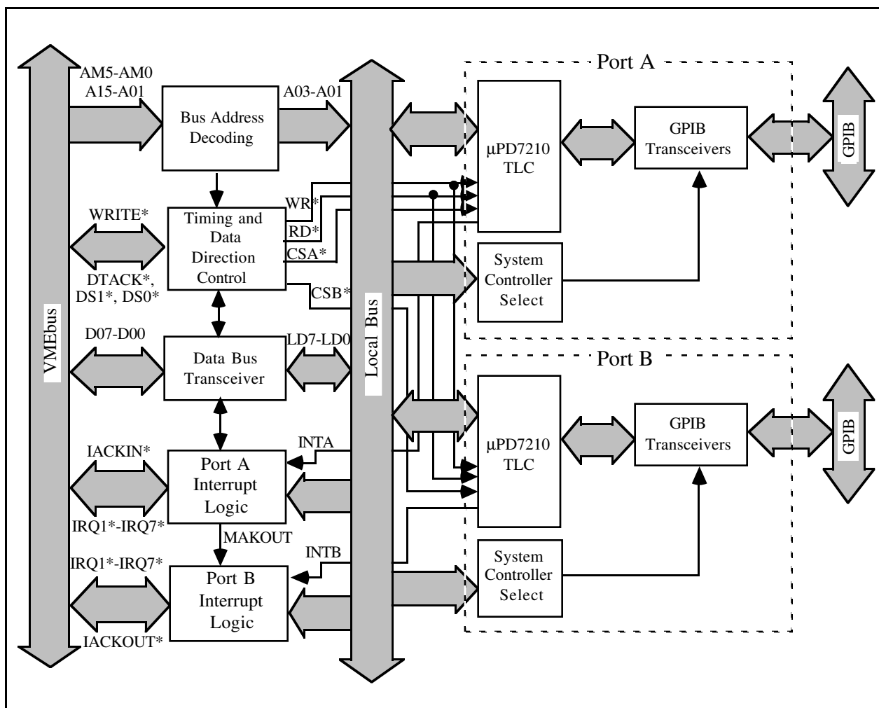
Figure 2-3. GPIB-1014DP Block Diagram
