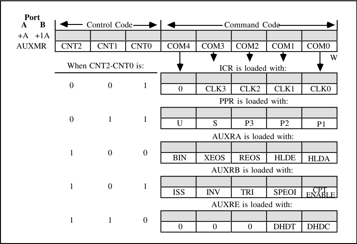
Figure 4-2. Writing to the Hidden Registers
