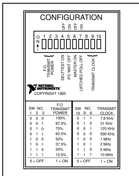
Figure 2-4. GPIO-110 Label
