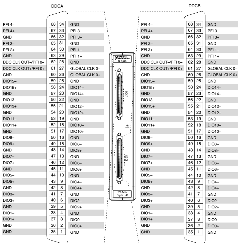
Figure 1. NI 6585/6585B Connector Pin Assignments
