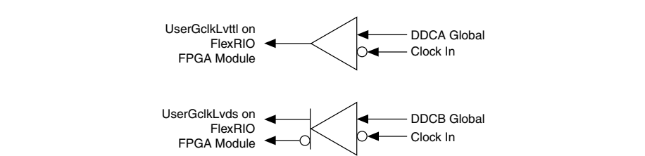
Figure 1. Clock Input (NI 6585 variant)
