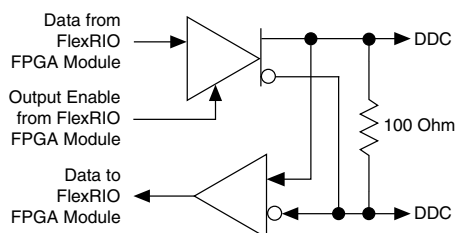
Figure 3. DIO <0..15> Data Channel, PFI <0..4>
