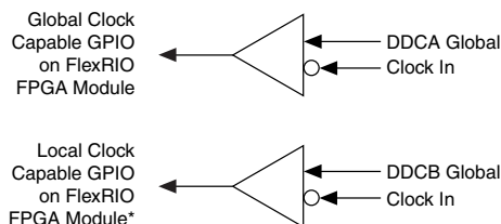
Figure 2. Clock Input (NI 6585B variant)
