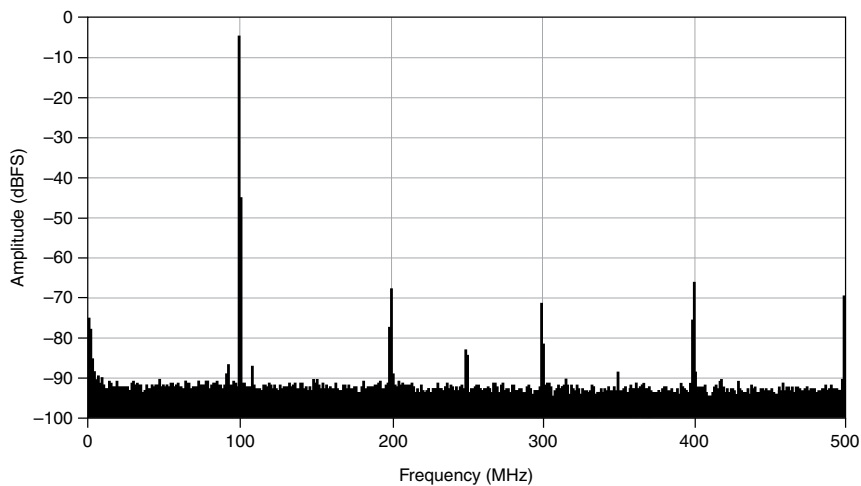
Figure 4. PCI-5153 Dynamic Performance, 2 V pk-pk Input Range, 100 MHz Input Signal, Measured
