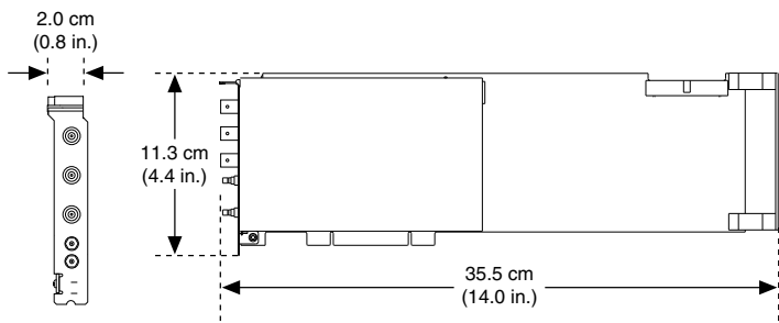
Figure 6. PCI-5153 Dimensions
