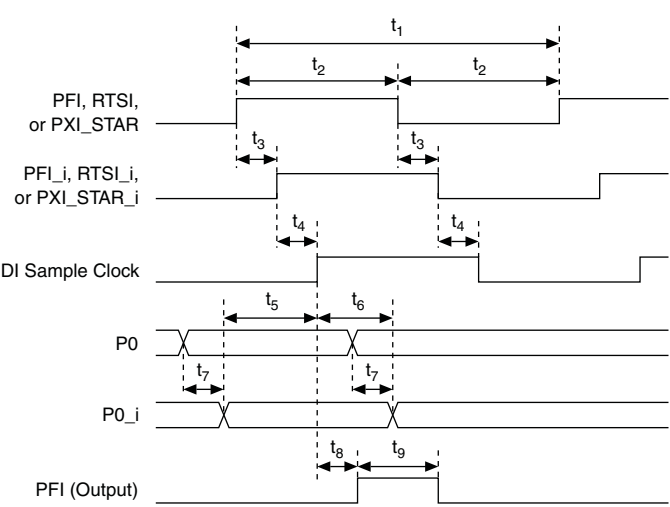
Figure B-38. Digital Waveform Acquisition Timing Delays
