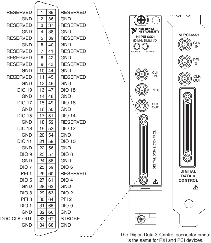
Figure 15. NI 6551/6552 Front Panel Connectors
