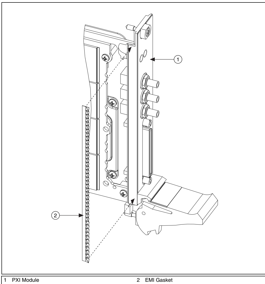
Figure 1. Gasket Placement on a PXI Module
