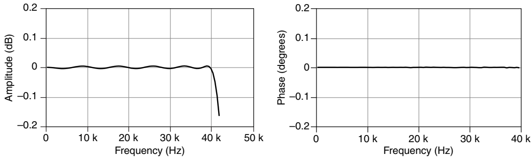
Figure 2. 100 kS/s Frequency Response, Measured
