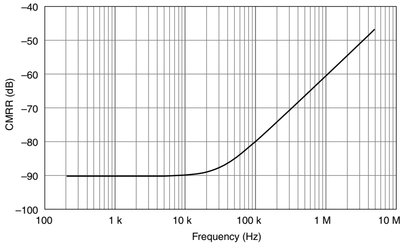
Figure 1. PXI-5922 CMRR with Differential Terminal Configuration, Measured
