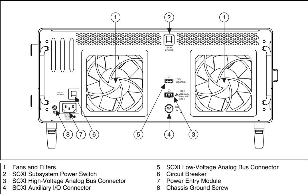
Figure 1-2. Rear View of the PXI-1011 Chassis
