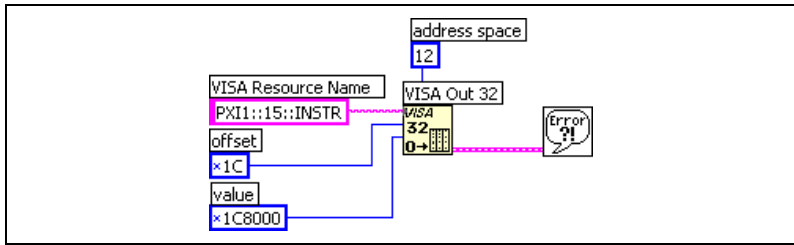
Figure 3. Adjusting the Frequency of the Clk10 Oscillator Using NI-VISA
