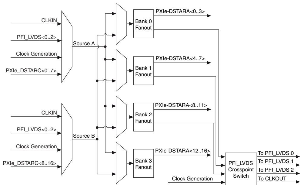
Figure 12. PXle-DStarA Topology
