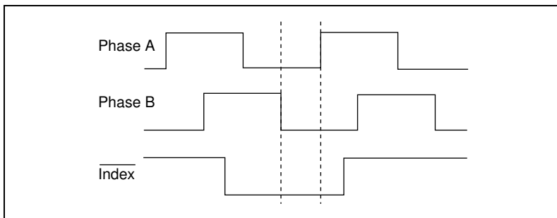
Figure 4-5. Quadrature Encoder Phasing Diagram
