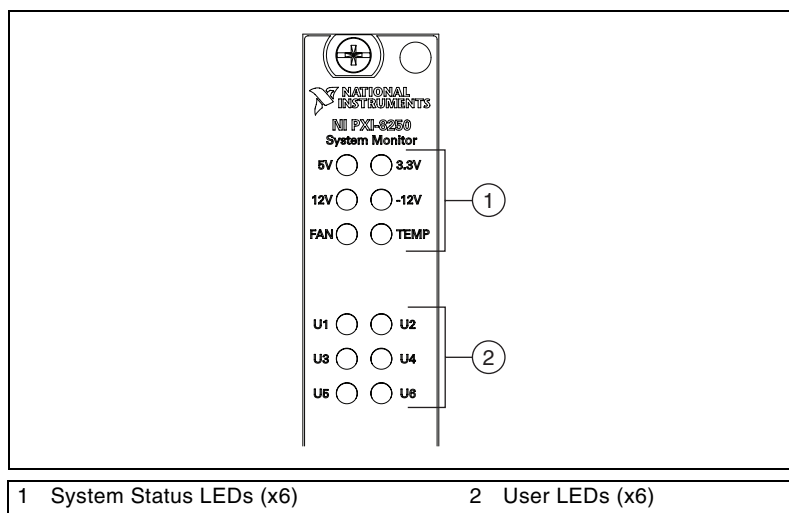
Figure 3-4. NI PXI-8250 Front Panel LED Diagram
