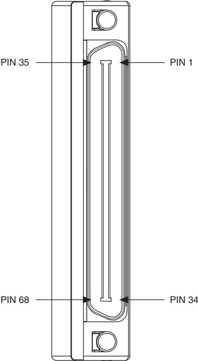
Figure 5. 68-Pin VHDCI Connector Pin Locations
