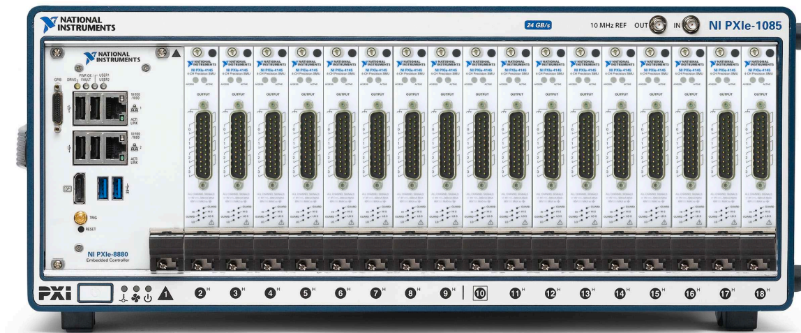
Figure 1. Using PXIe-414x, you can add up to 68 SMU channels in a single 4U, 19-inch PXI chassis. The PXIe-4162 and PXIe-4163 extend this to 204 and 408 channels, respectively.
