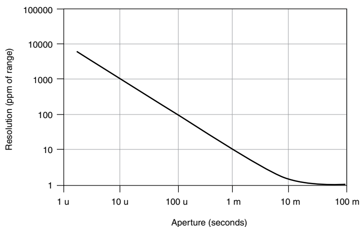
Figure 2. Noise and Resolution versus Measurement Aperture, Typical
