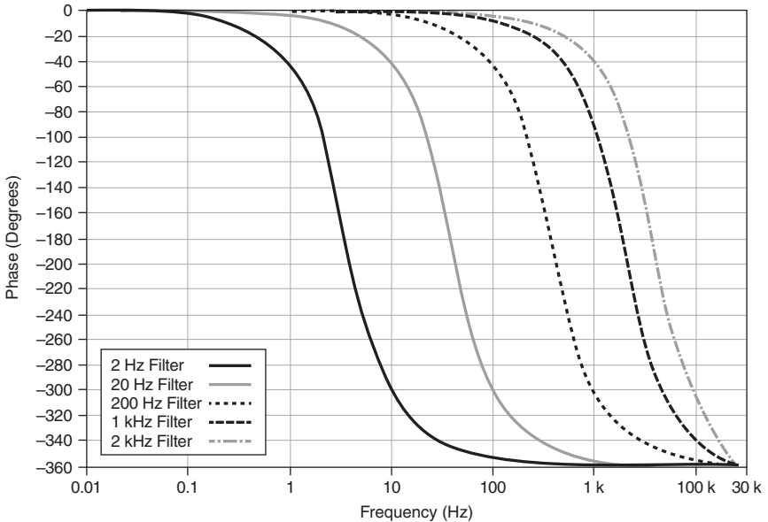
Figure 3. Phase Response
