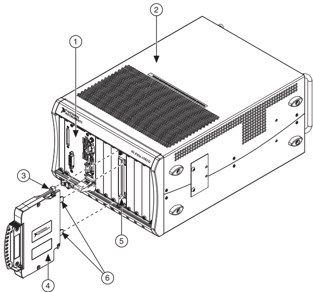
Figure 8. Installing the Terminal Block on the Module
