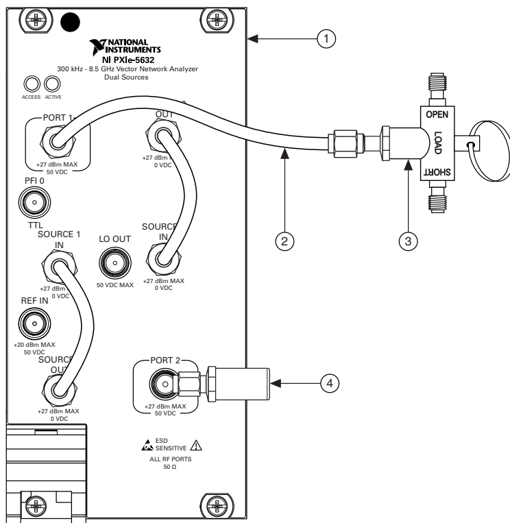
Figure 7. System Dynamic Range Verification Equipment Setup
