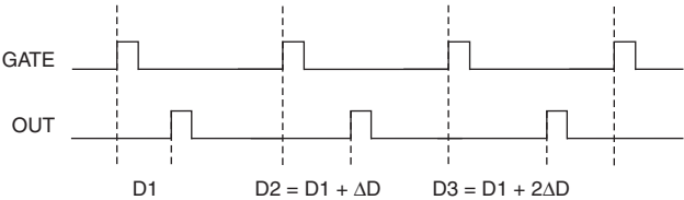
Figure 7-29. Pulse Generation for ETS
