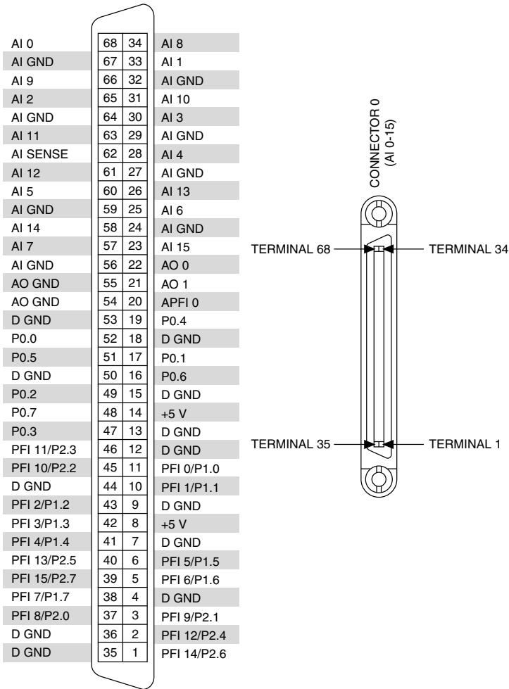
Figure 9. NI PCI/PCIe/PXI/PXLe-6251 Pinout
