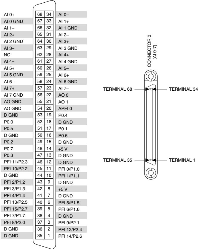
Figure 6. NI PXIe-6356 Pinout
