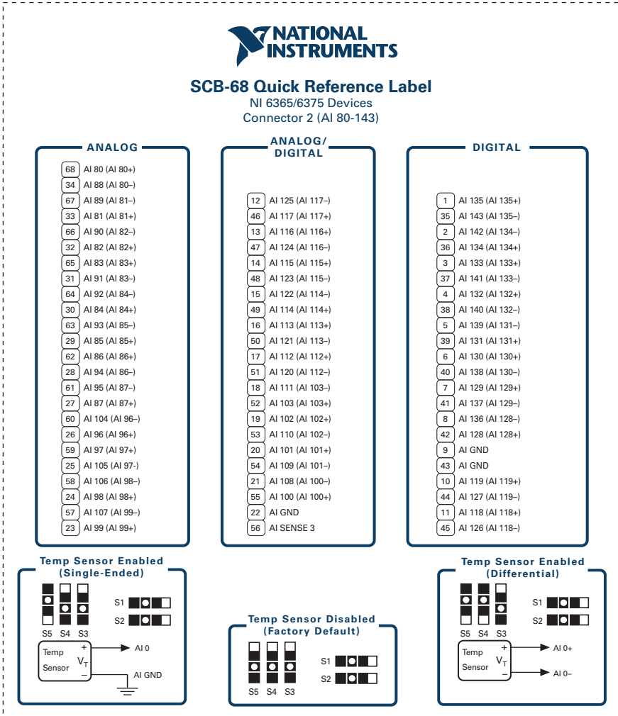
Figure 10. NI 6365/6375 Connector 2
