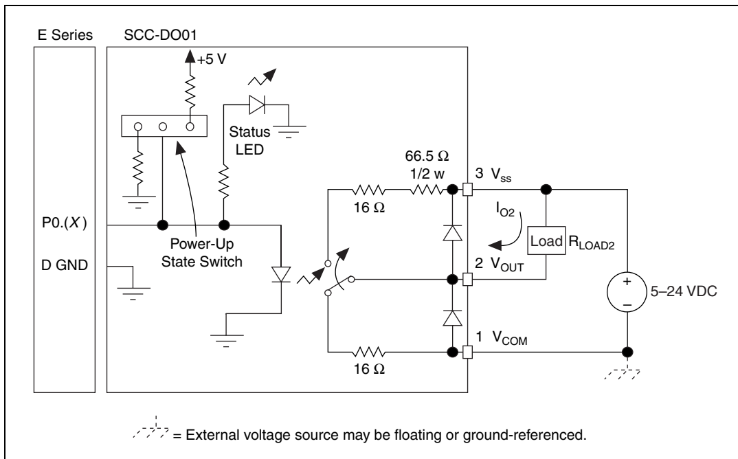
Figure 2. Connecting a Load R_{LOAD2} to V_{OUT} and V_{SS} (Configuration 2)
