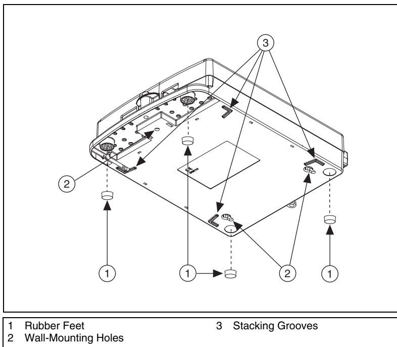
Figure 4. SCC-68 Mounting Features
