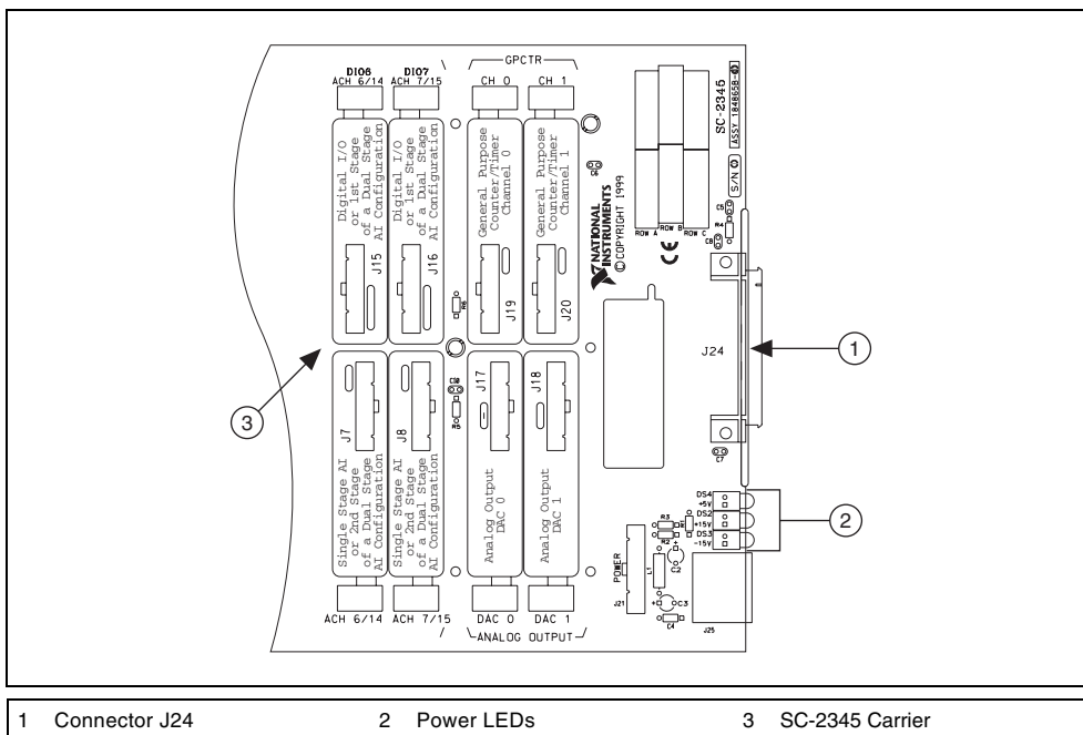
Figure 1. Connector J24 Location The chassis ground terminal on the SC-2345/2350 carrier and the electromagnetic interference (EMI) gasket attached to the strain relief of the SC-2345 connector block are used to ground a floating source (1 mA maximum). Do not use these terminals as safety earth grounds. For more information about the SC-2345/2350 carrier, refer to the SC-2345/2350 Carrier User Manual .
