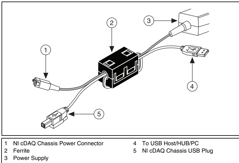
Figure 2. Ferrite Closed Over Looped Cables
