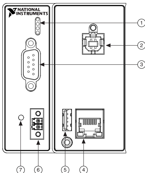
Figure 2. cRIO-9063 Front Panel
