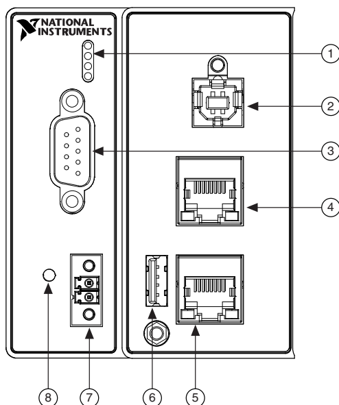
Figure 2. cRIO-9065 Front Panel
