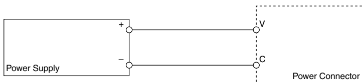
Figure 3. cRIO-9065 Power Connections
