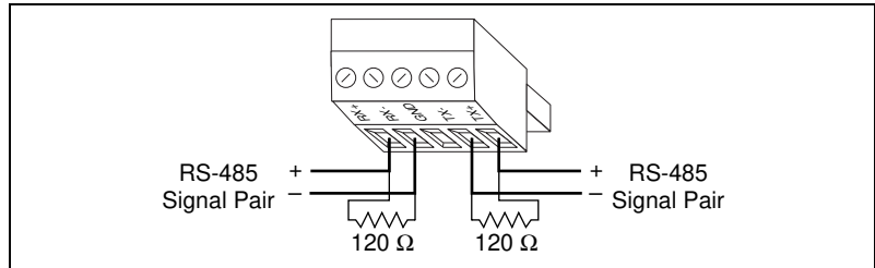
Figure 2-12. Terminating RS-485 Using the Combicon Adapter
