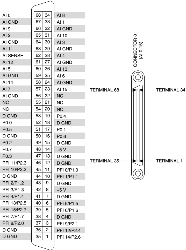
Figure 8. NI PCI/PXI-6220 Pinout
