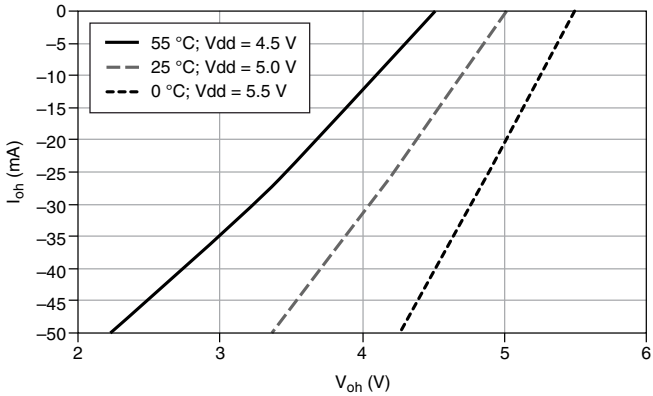
Figure 4. DIO (P0.<0..7>): I oh versus V oh
