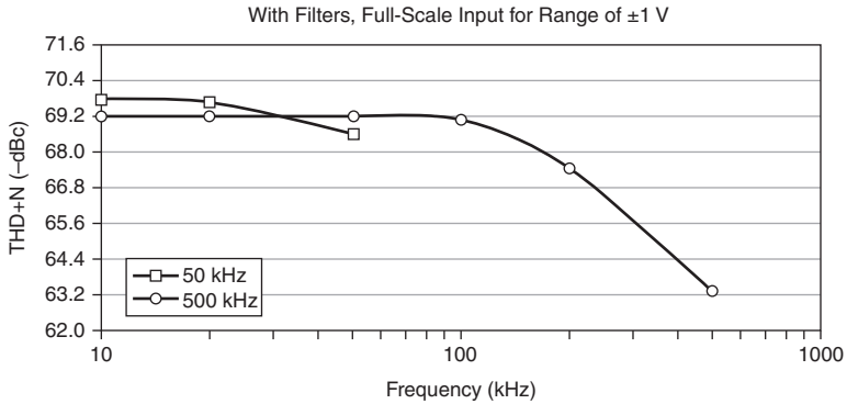
Figure 6. NI 6120 THD+N with Filters
