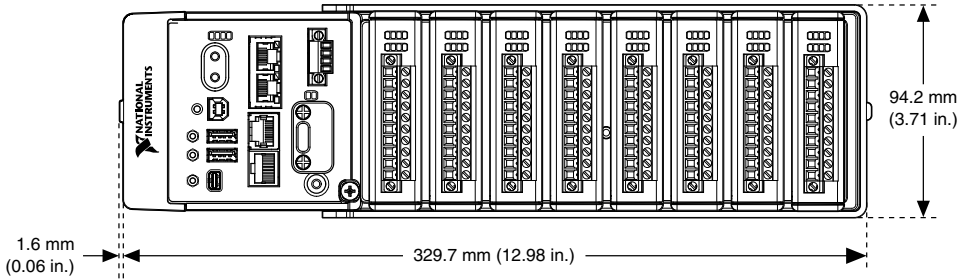
Figure 7. cRIO-9036 Module Immobilization Accessory Dimensions
