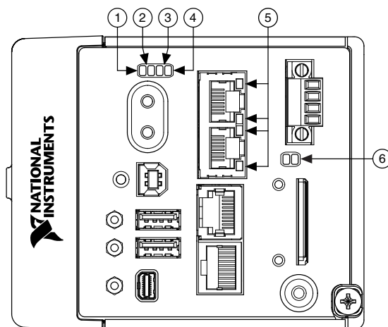
Figure 5. cRIO-9036 LEDs
