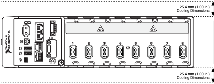
Figure 11. cRIO-9036 Cooling Dimensions
