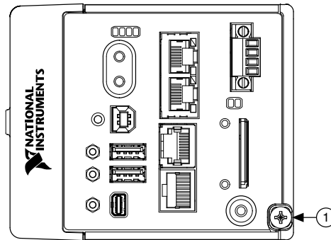
Figure 6. cRIO-9036 Chassis Grounding Screw
