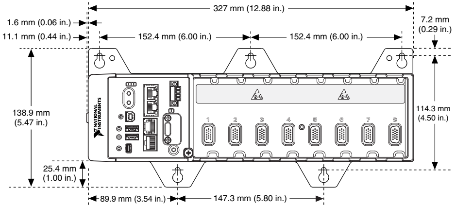
Figure 15. cRIO-9036 Panel Mounting Dimensions
