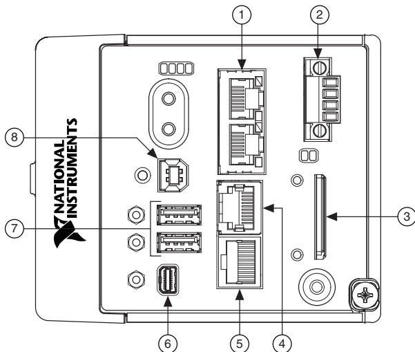
Figure 1. cRIO-9036 Ports and Connectors
