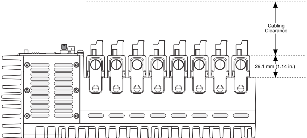
Figure 12. cRIO-9036 Cabling Clearance
