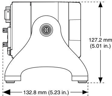
Figure 17. cRIO-9036 Desktop Mounting Side Dimensions
