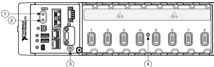
Figure 3. cRIO-9036 Buttons
