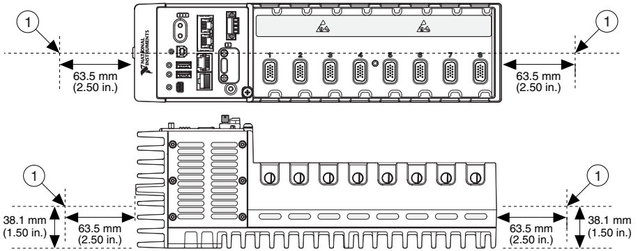
Figure 13. cRIO-9036 Ambient Temperature Location
