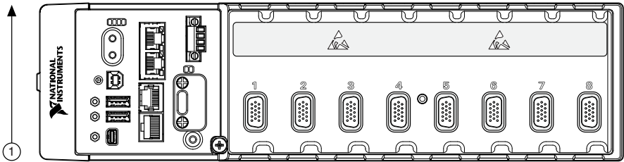
Figure 8. cRIO-9036 Horizontal Mounting
