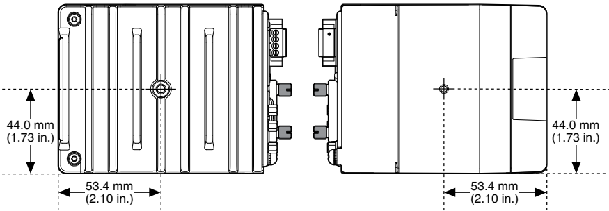
Figure 10. cRIO-9036 Side Dimensions
