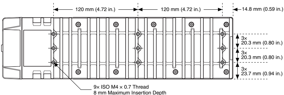
Figure 14. cRIO-9036 Surface Mounting Dimensions
