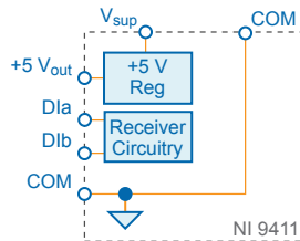
Figure 1. NI 9411 Input Circuitry
