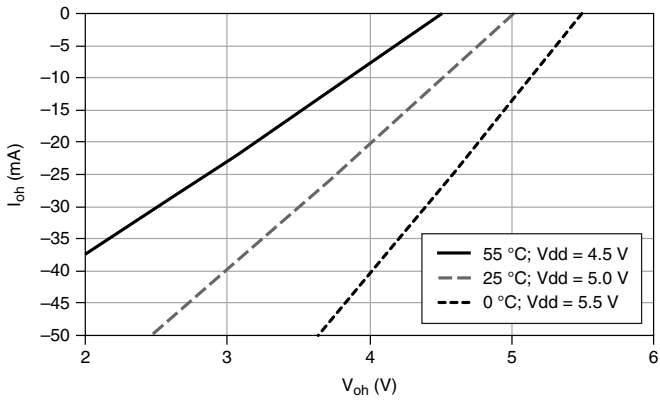
Figure 5. PFI <0..7>/P1: I_{oh} versus V_{oh}
