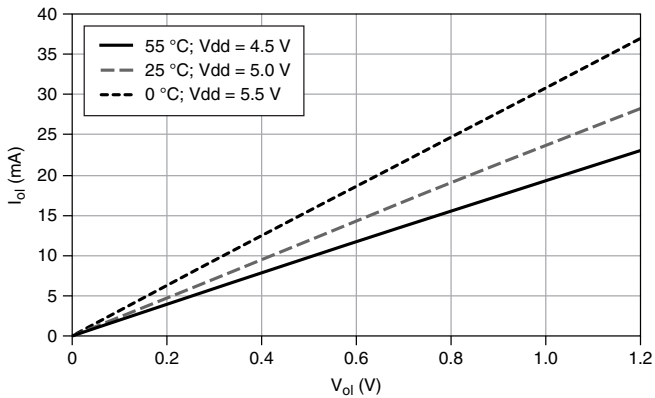
Figure 7. P1.<0..7> : I_{ol} versus V_{ol}
