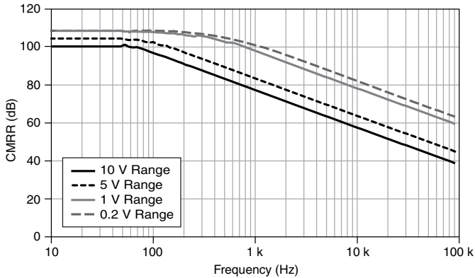
Figure 3. AI CMRR
