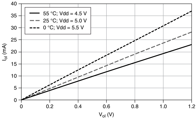
Figure 8. Digital I/O (PFI <0..15>/P1/P2): I_{OI} versus V_{OI}
