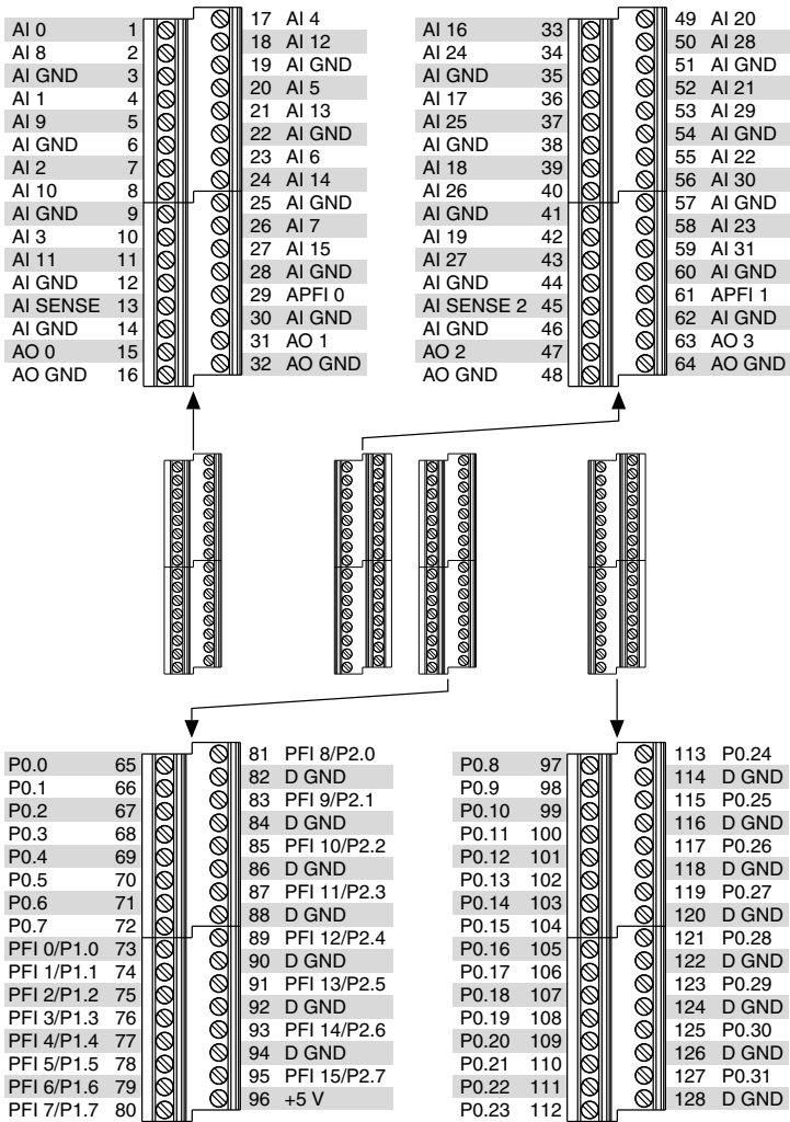
Figure 11. NI USB-6289 Screw Terminal Pinout
