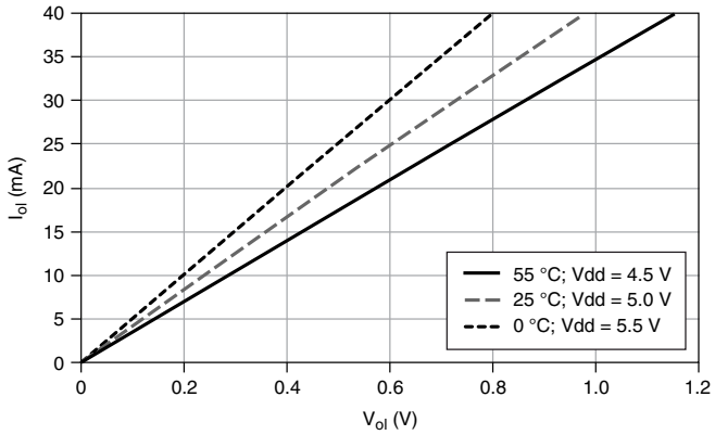
Figure 7. Digital I/O (P0.<0..31>): I_{ol} versus V_{ol}
