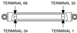
CONNECTOR 0 (AI 0–15)
