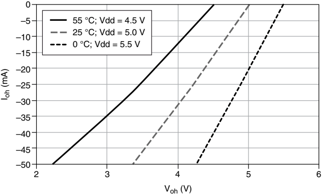
Figure 5. Digital I/O (P0.<0..31>): I oh versus V oh
