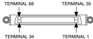
CONNECTOR 1 (AI 16–31)
