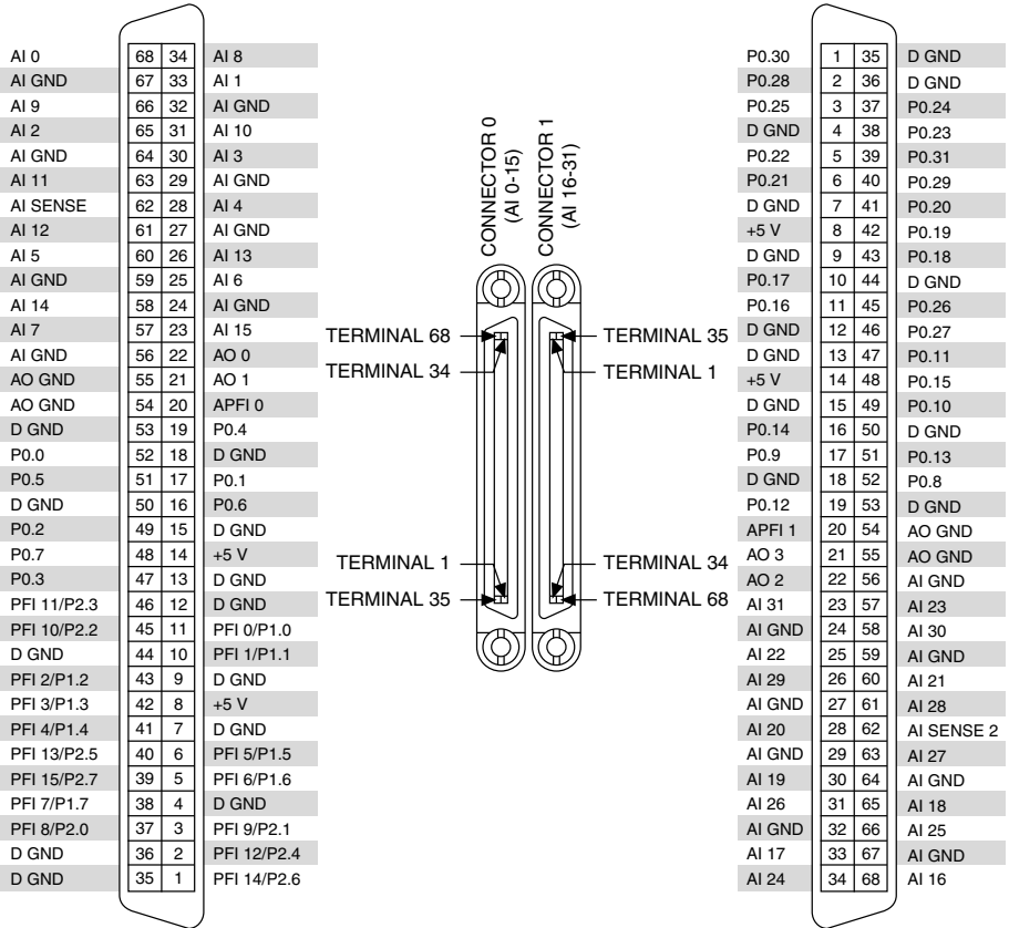
Figure 9. NI PCI/PXI-6289 Pinout
