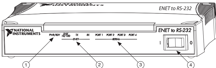
Figure 2. Four-Port Serial ENET Hardware LEDs
