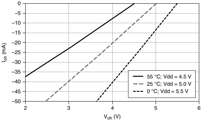
Figure 6. P1.<0..15>/P1/P2: I_{oh} versus V_{oh}
