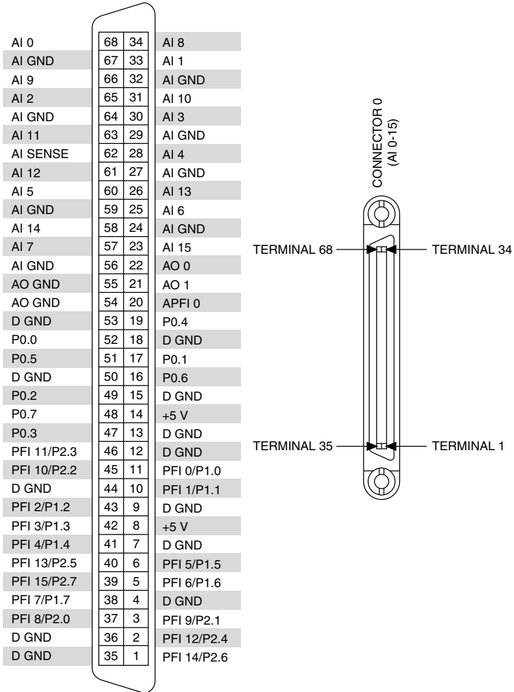
Figure 9. NI PCI/PCIe/PXI/PXLe-6251 Pinout
