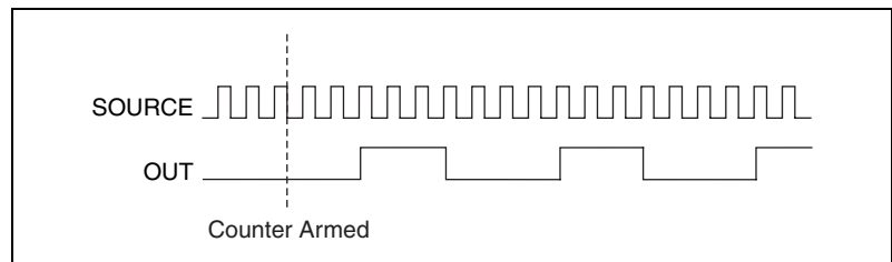
Figure 7-25. Continuous Pulse Train Generation
