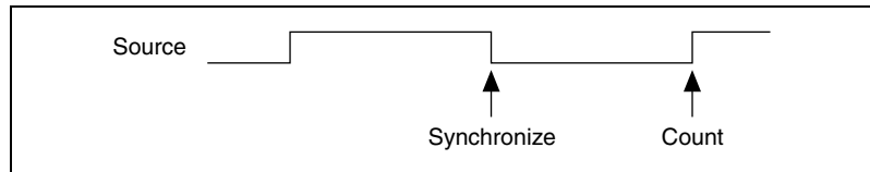
Figure 7-35. Other Internal Source Mode
