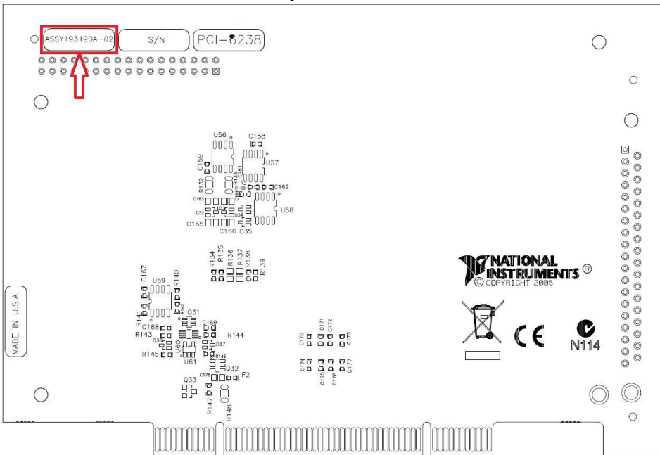
PCI-6232/6233/6238/6239 – Secondary Side
