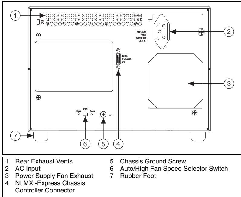
Figure 1-2. Rear View of the NI PXI-1033 Chassis
