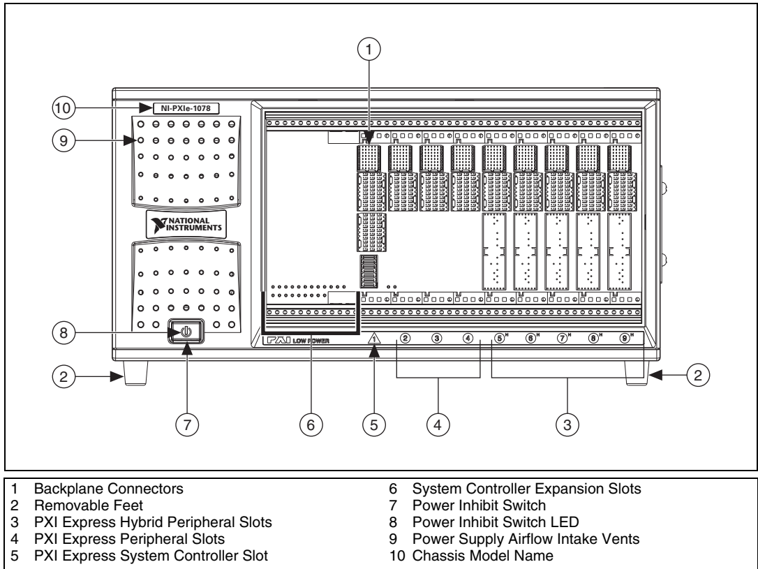
Figure 1-1. Front View of the NI PXIe-1078 Chassis
