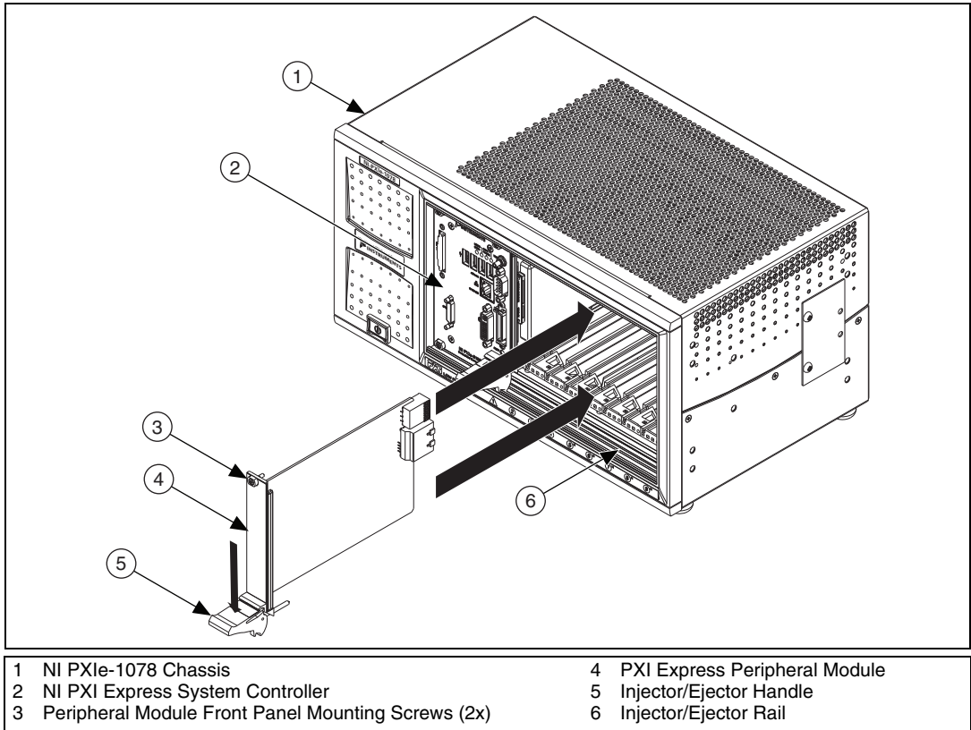
Figure 2-6. Installing PXI, PXI Express, or CompactPCI Peripheral Modules
