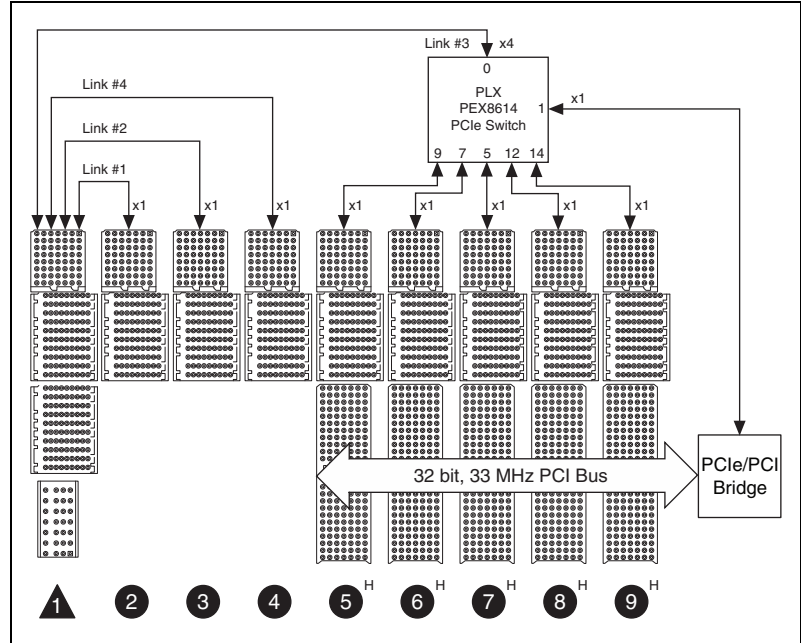
Figure 1-4. NI PXIe-1078 Backplane Architecture
