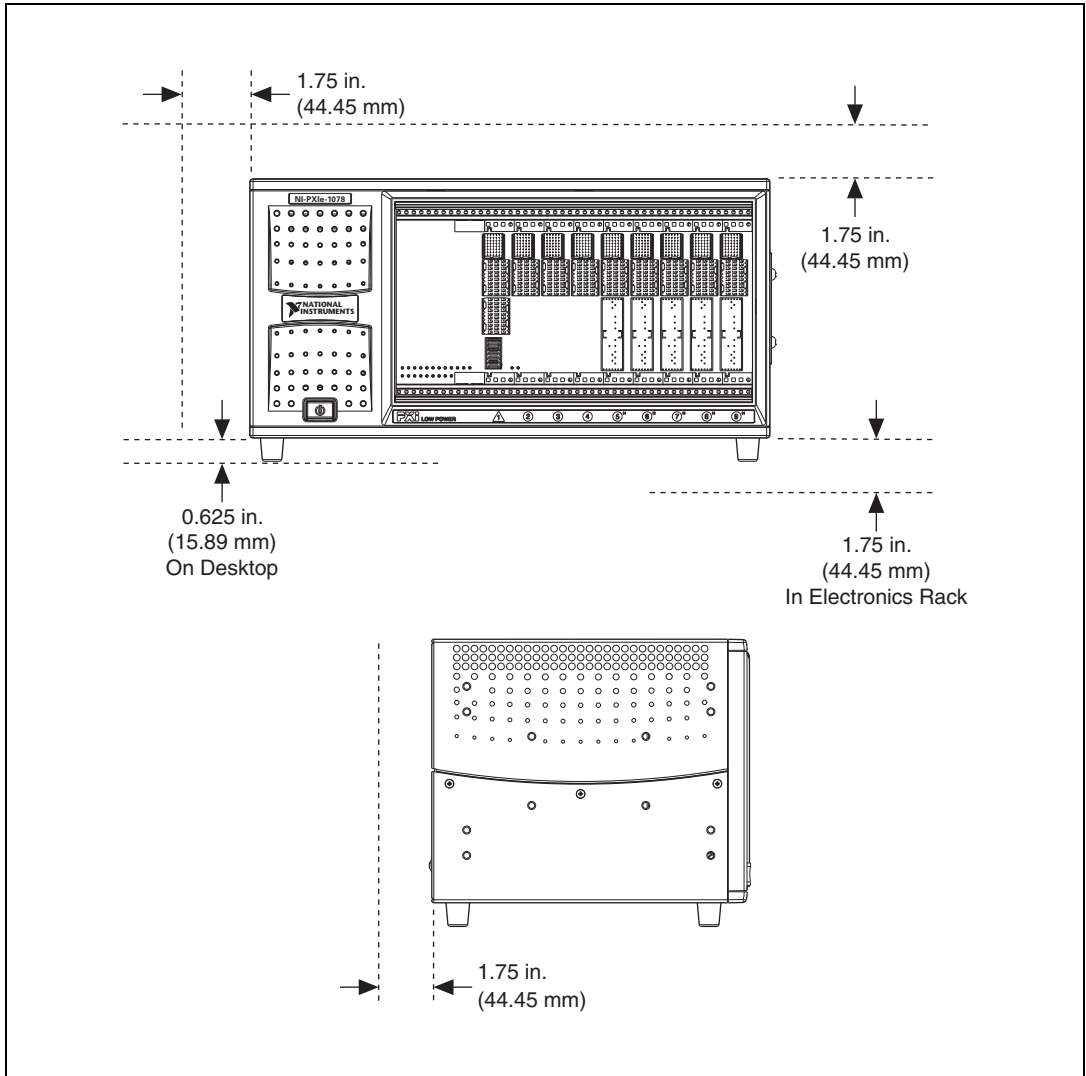
Figure 2-3. NI PXIe-1078 Cooling Clearances
