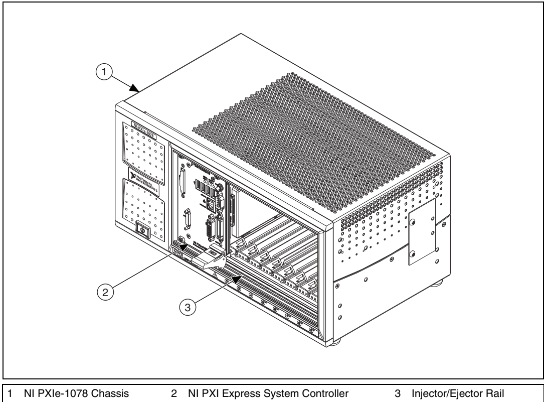
Figure 2-5. NI PXI Express System Controller Installed in an NI PXIe-1078 Chassis
