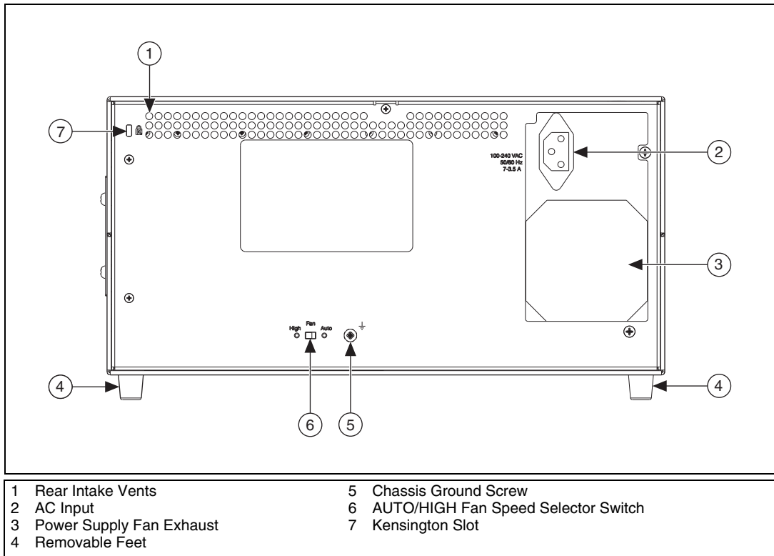
Figure 1-2. Rear View of the NI PXIe-1078 Chassis
