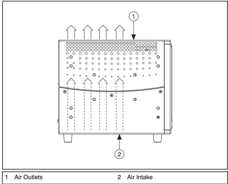
Figure 2-1. NI PXIe-1078 Module Cooling Airflow Side View
