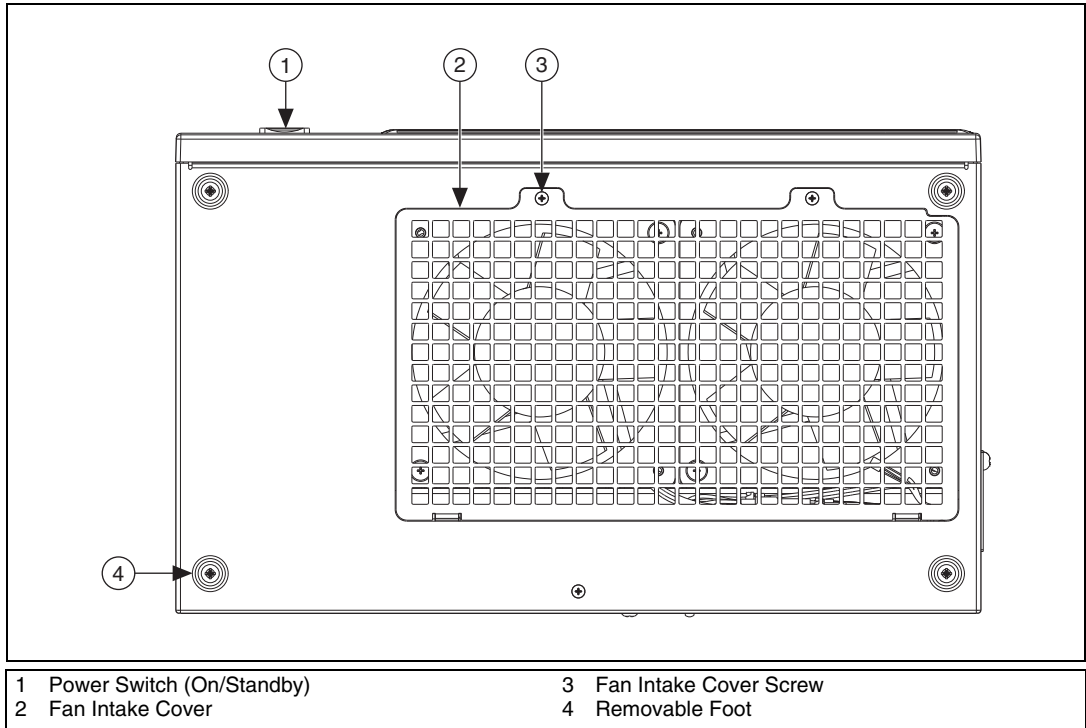
Figure 1-3. Bottom View of the NI PXIe-1078 Chassis
