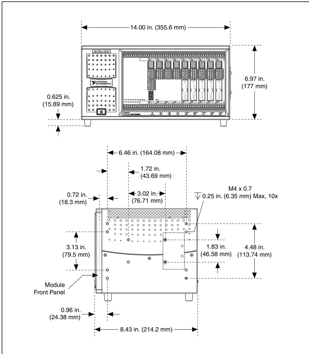
Figure A-1. NI PXIe-1078 Chassis Dimensions (Front and Side)
