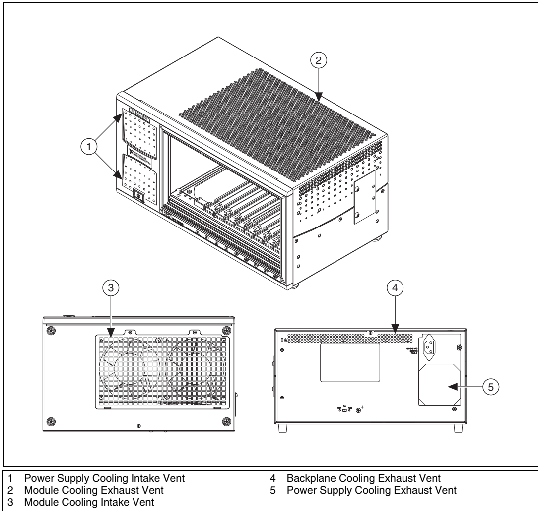
Figure 2-2. NI PXIe-1078 Vents
