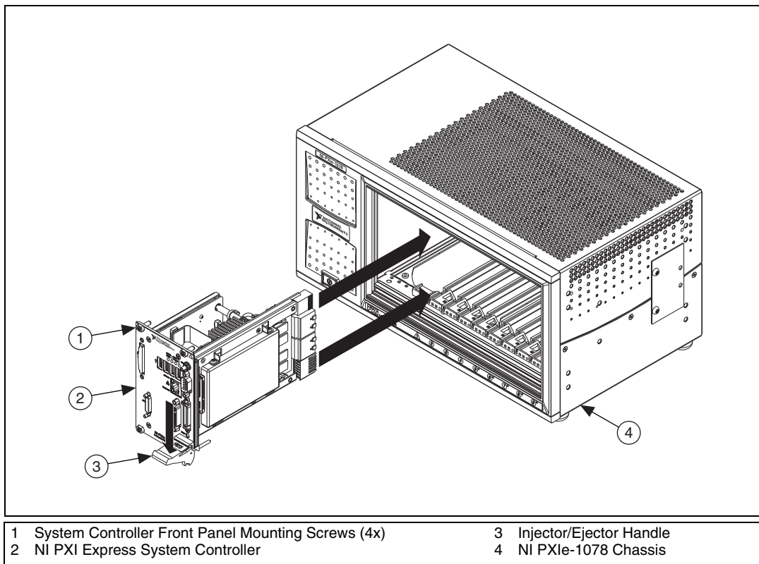
Figure 2-4. Installing a PXI Express System Controller
