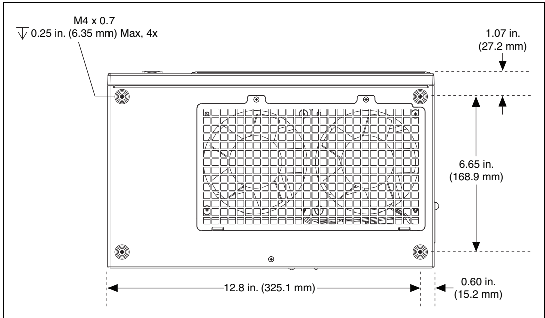
Figure A-2. NI PXIe-1078 Chassis Dimensions (Bottom)
