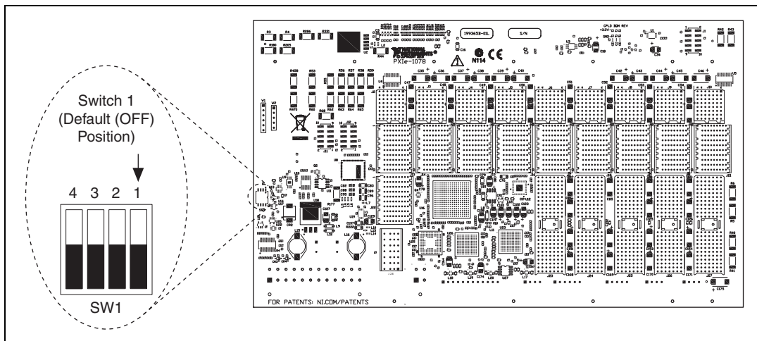
Figure 2-7. Switch 1 of SW1
