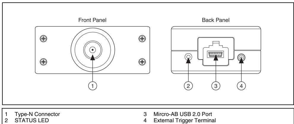
Figure 4. NI USB-5681 Front and Back Panel
