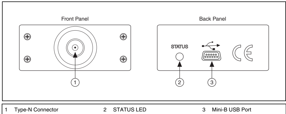
Figure 3. NI USB-5680 Front and Back Panel
