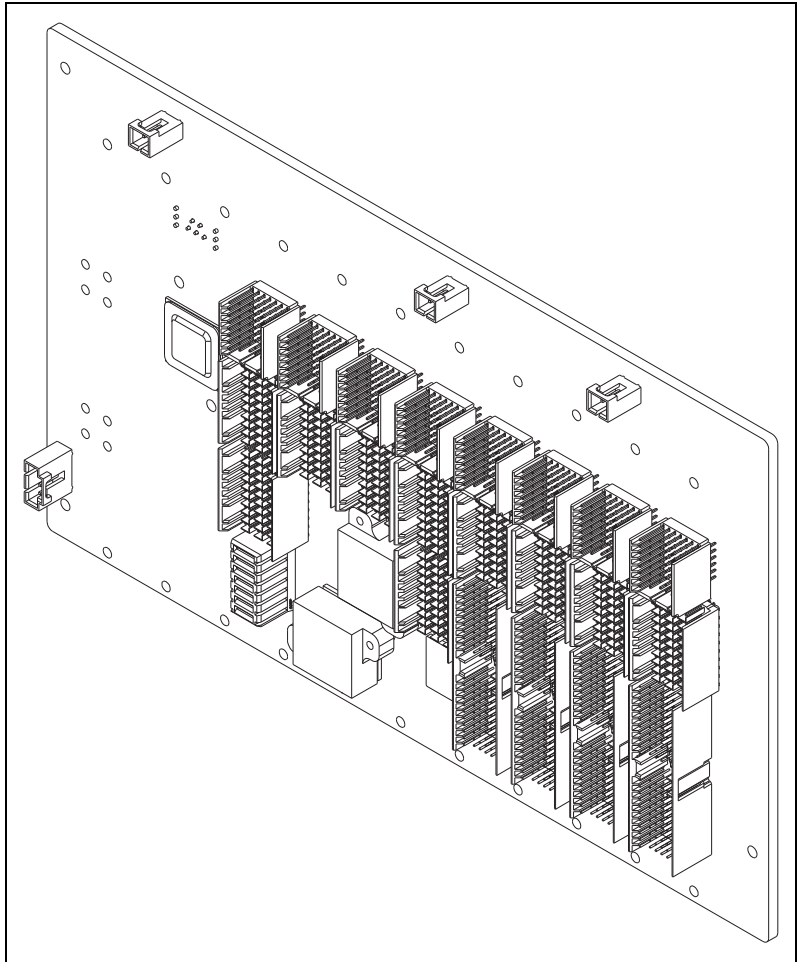
Figure 1. 8-Slot NI PXIe-1082 Backplane
