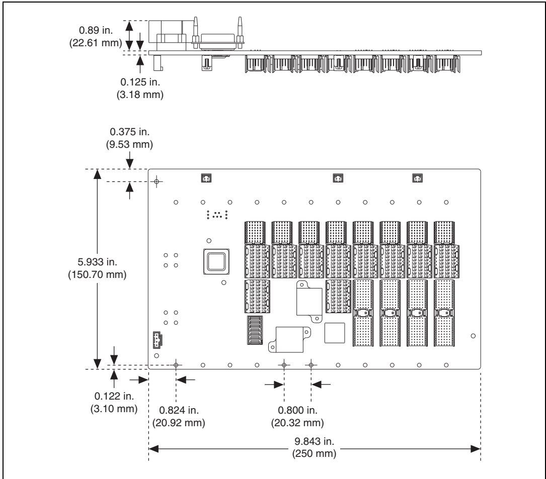
Figure 8. Dimensions
