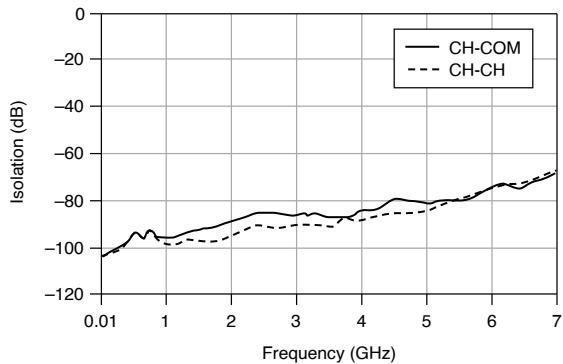
Figure 3. Isolation, Typical
