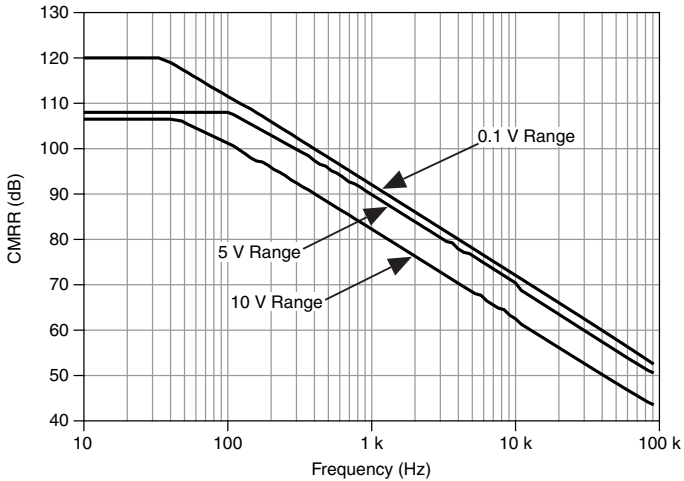
Figure 1. AI <0..31> CMRR
